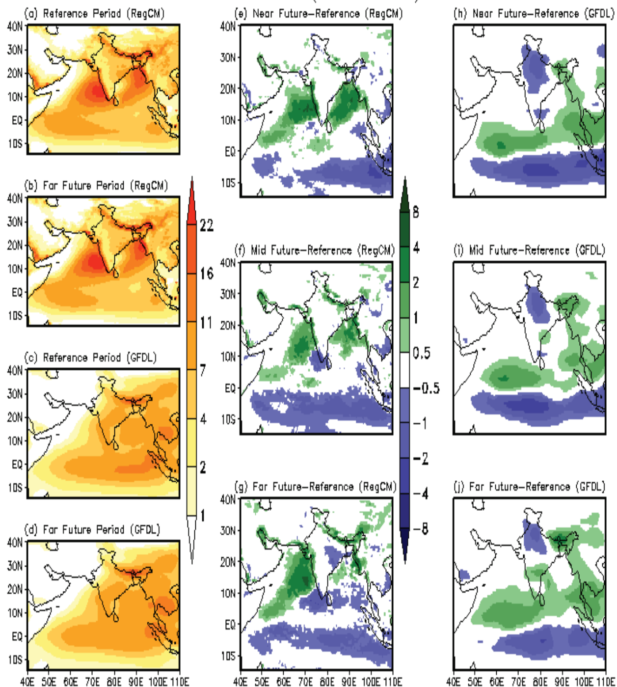
Figure 13: Climatological mean JJAS rainfall (mm/day) in the vicinity of Indian summer monsoon region during present (1975 to 2004), near future (2010 to 2039), mid future (2040 to 2069) and far future (2070 to 2099) in RCP4.5 scenarios
