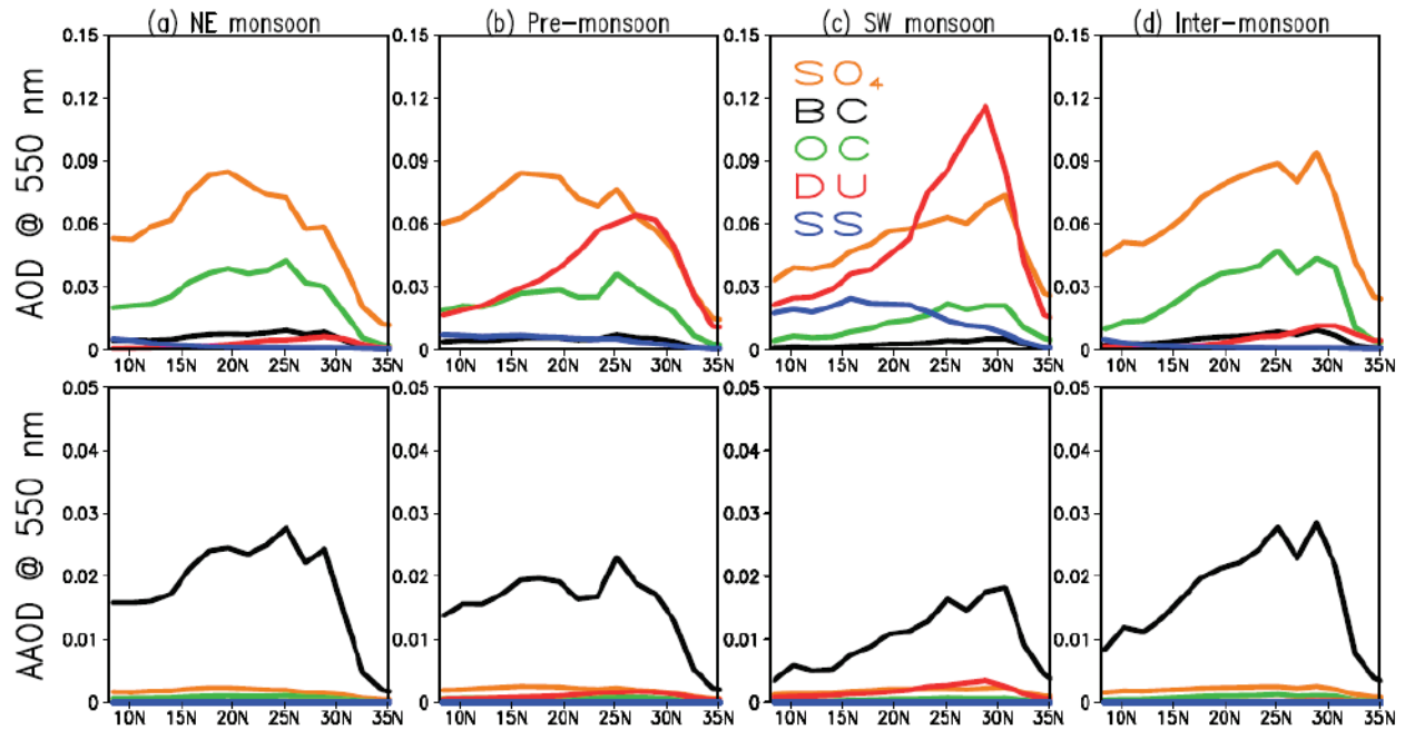
Figure 32: Seasonal zonal mean (68E-98E) ECHAM model simulated contributions by different aerosols species to aerosol optical depth (AOD, top panel) and
