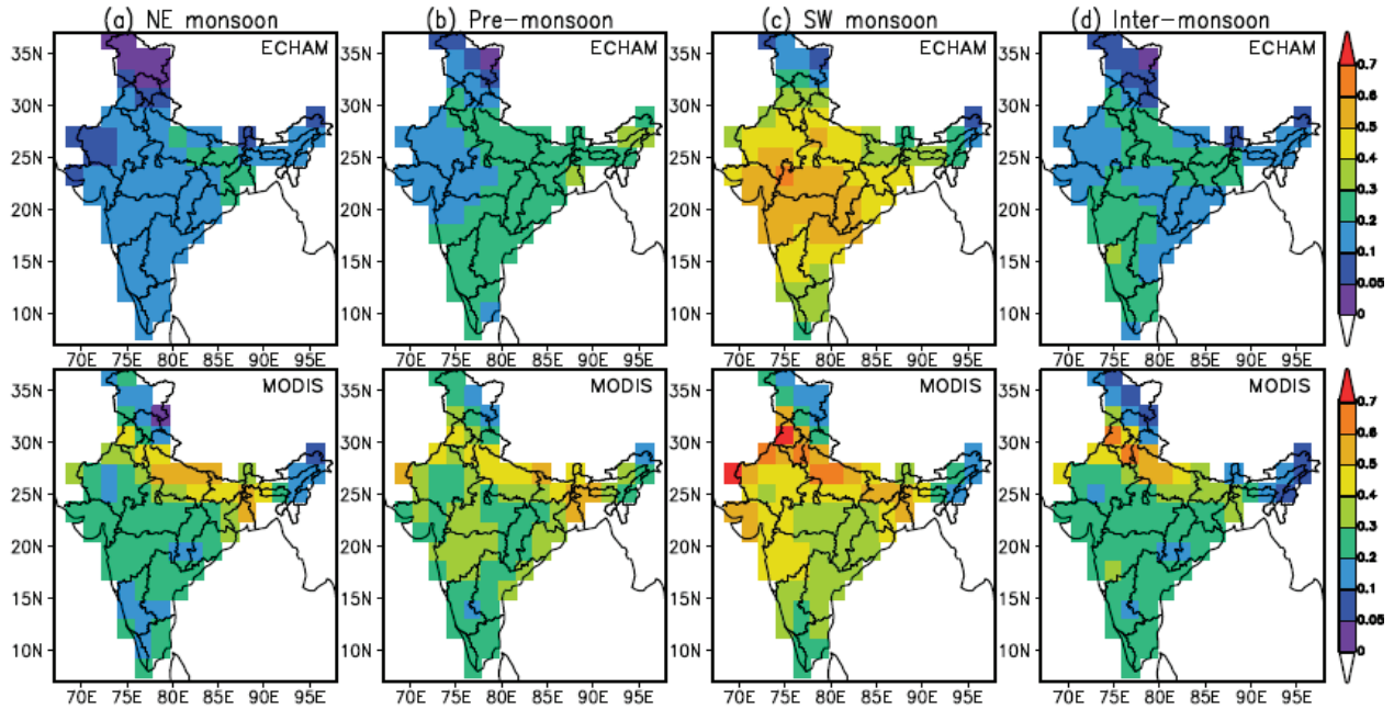
Figure 31: Seasonal mean distribution of ECHAM model simulated aerosol optical depth at 550 nm and MODIS satellite retrievals (January 2001 to December 2005)
