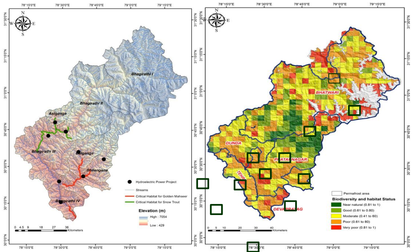
Figure 4.11. Long term monitoring areas selected for aquatic and terrestrial ecosystems for annual ecosystem health assessment in Bhagirathi Basin, Uttarakhand
