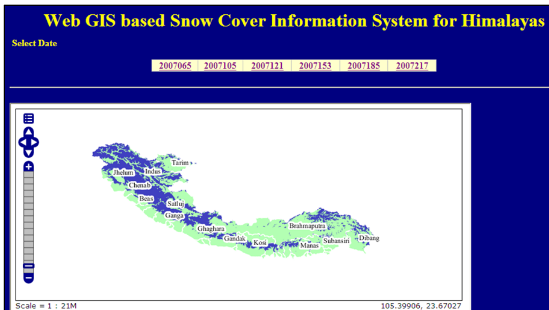
Figure 2.2. Web-GIS based snow cover information for Himalayas
