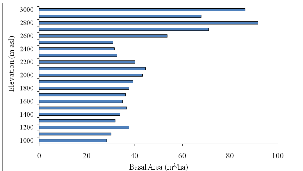
Figure 11. Trends of basal cover (m 2 /ha) of tree species along altitudinal range in Western Himalaya
