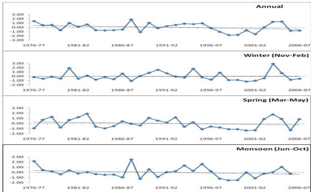
Figure 2.22. Trends in seasonal/annual flow in Tawi river at Jammu
