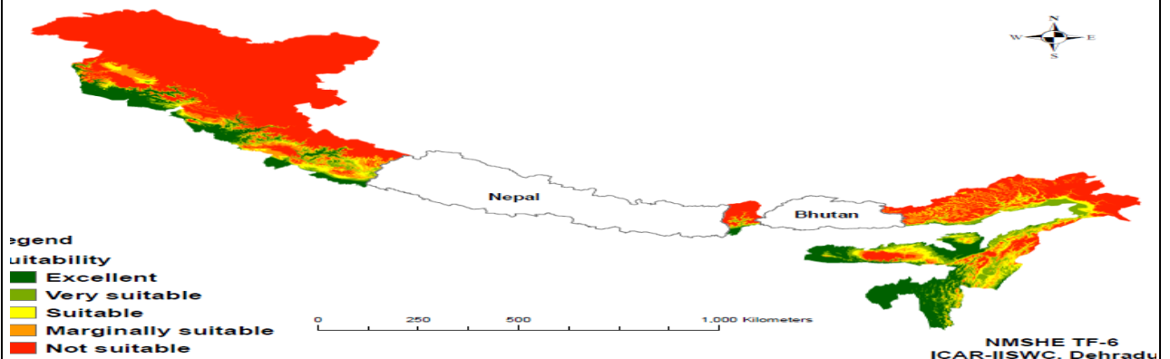
Base Map of climate suitability for growing maize in IHR
